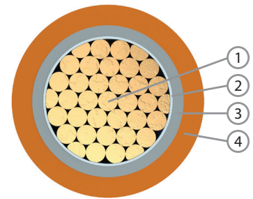
Component 1. Plain Annealed Copper Wire 2. Mica Tape 3. Cross-linked Polyethylene Compound 4. Low Smoke Zero Halogen (LSZH) Compound
