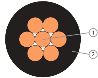
Component 1. Plain Annealed Copper Wire 2. Cross-linked Polyolefin Low Smoke Zero Halogen Compound
