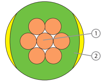
Component 1. Plain Annealed Copper Wire 2. PV Compound
